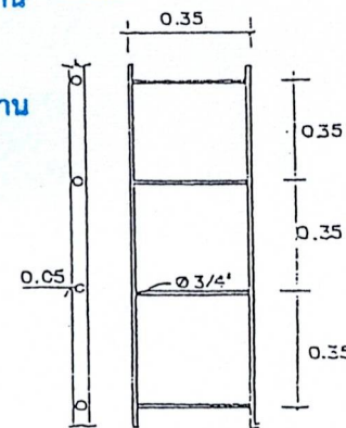
DETAIL LADDER
