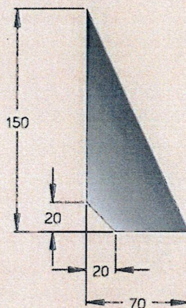
SUPPORT POLE DETAIL SCALE 1: 4
